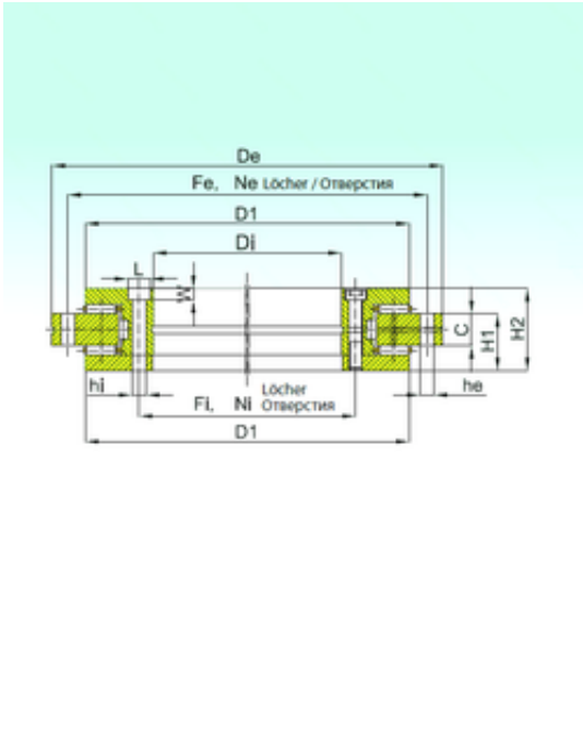
YRTS 395 Bearing 2D drawings and 3D CAD models
